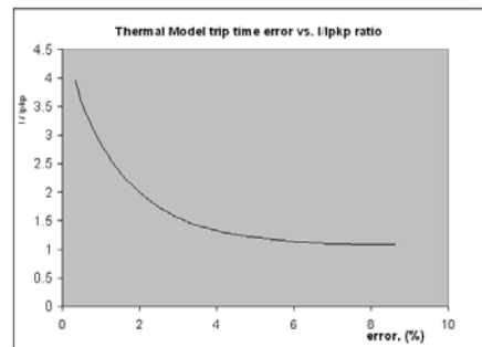
The graph shows the trip time error with respect to the ratio of cable load and thermal model pickup setting. With a smaller I/pkp ratio, the time error tends to be higher, as accumulated through the logarithmic formula, the measurement error, and the time of measurement. For higher I/pkp ratios, the time to trip is substantially more accurate. Each point on the graph represents a trip time error, with the I/pkp ratio kept constant during the test.
