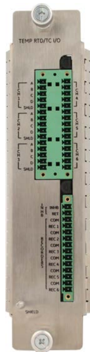
Figure 2: Rear view of the Temperature Monitor I/O module
